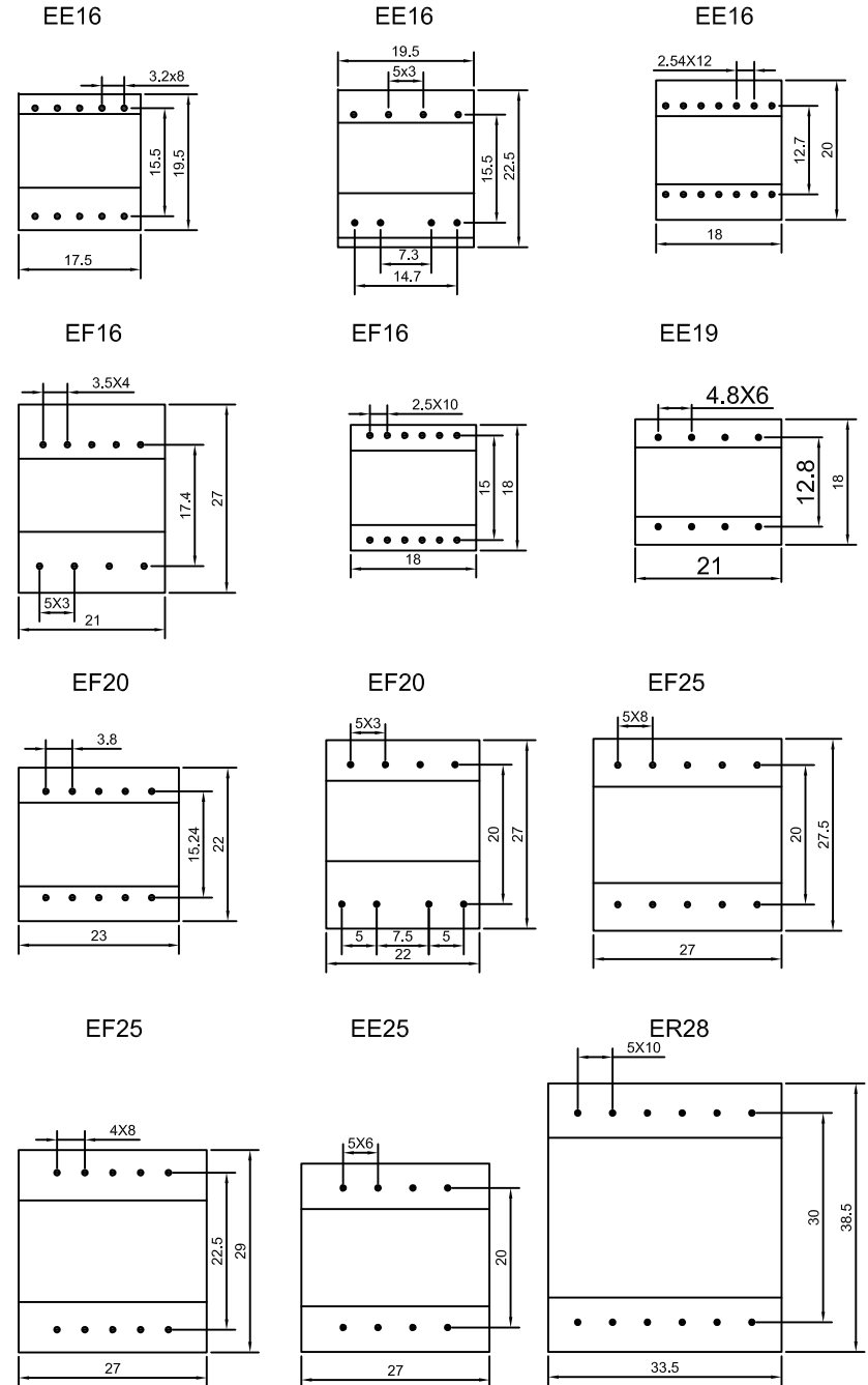
卧式结构(Horizontal structure)
